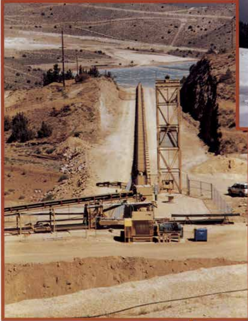
▲ Shop fabricated and field erected 4,900 ft. overland conveyor system for a Northern Nevada mine.
