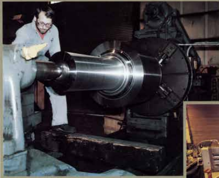
▶ Machining of a press roll shaft in a 80 in. x 30 ft. lathe.
