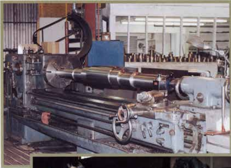
◀ Machining eccentric shaft for large jaw crusher for a mining company in northern Nevada.
